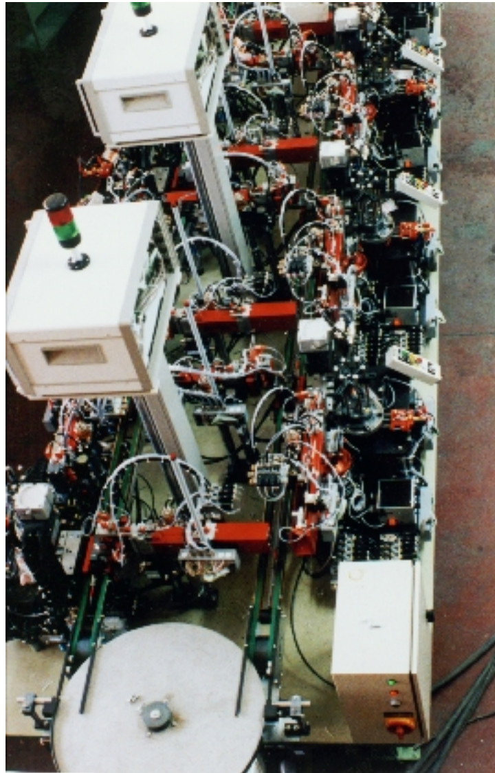
HARMONICA ASSEMBLY MACHINE
