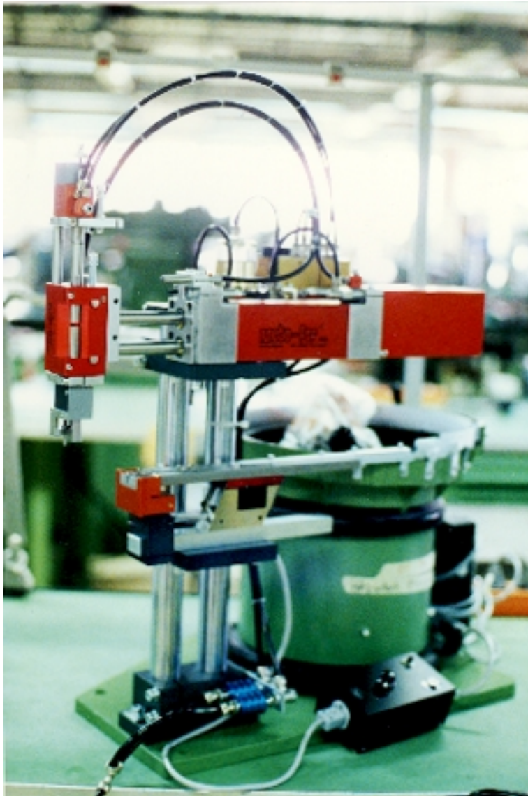
PICK & PLACE WITH BOWL FEEDER
