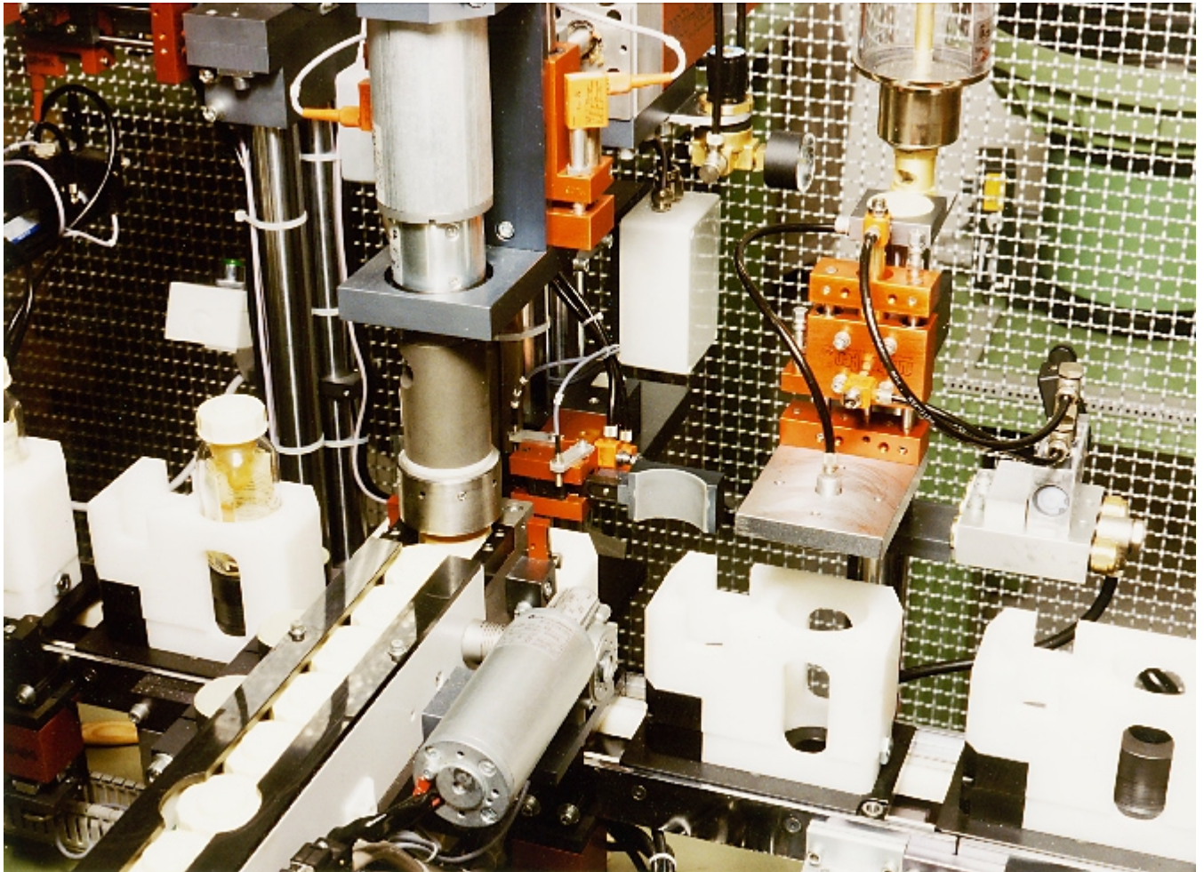
NURSING BOTTLE ASSEMBLY MACHINE
